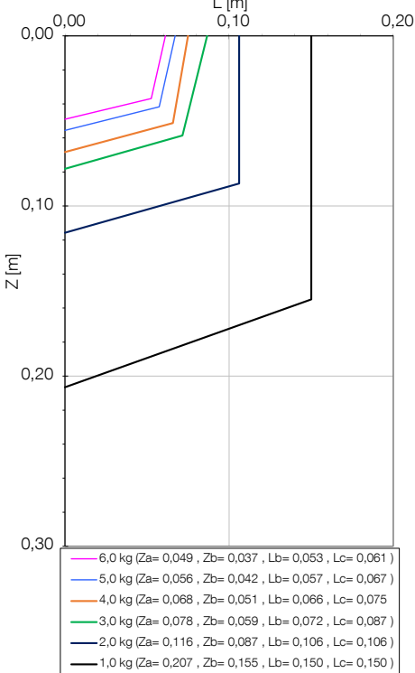
Load Diagram IRB 910SC - 3 / 0.45
