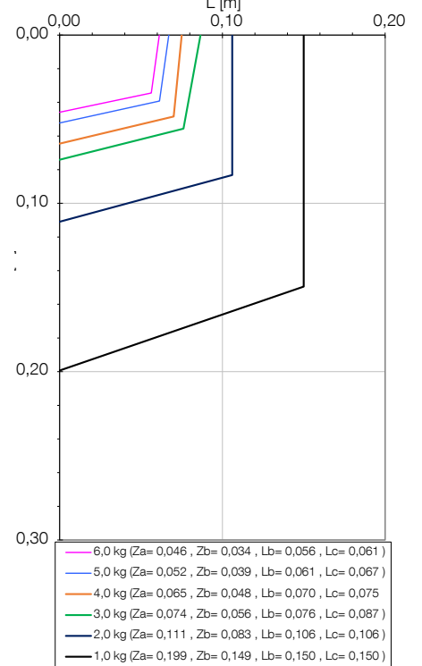
Load Diagram IRB 910SC - 3 / 0.65
