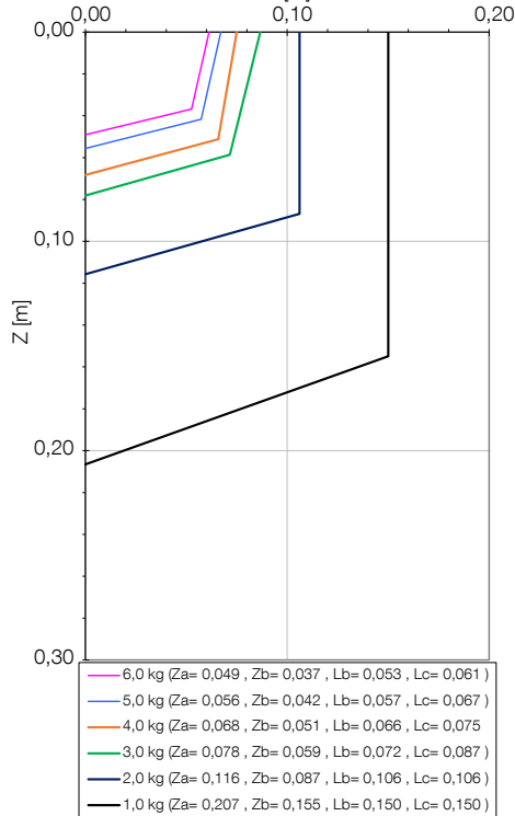
Load Diagram IRB 910SC - 3 / 0.55
