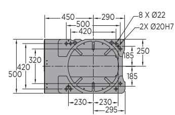
VIEW C
