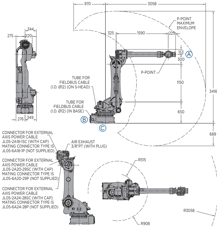
VIEW A
