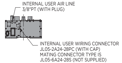
VIEW C
